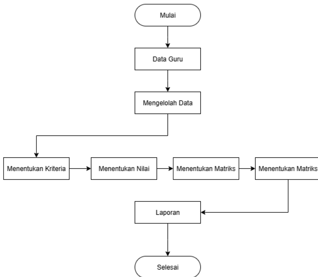
Gambar 3.2 Activity Diagram
